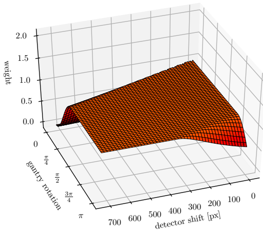
Parker weights before learning
