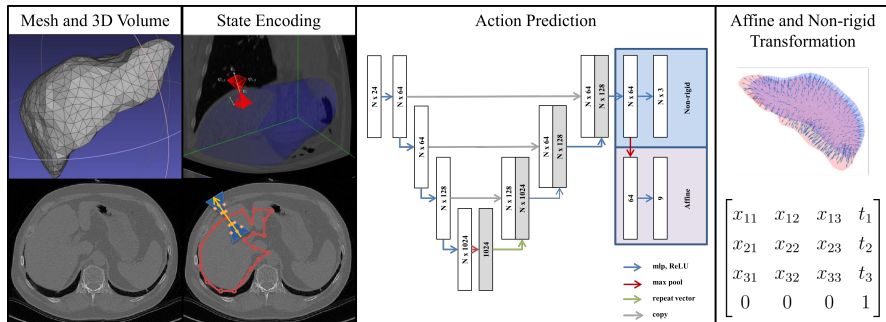
Action prediction pipeline for 3D point cloud based organ segmentation
